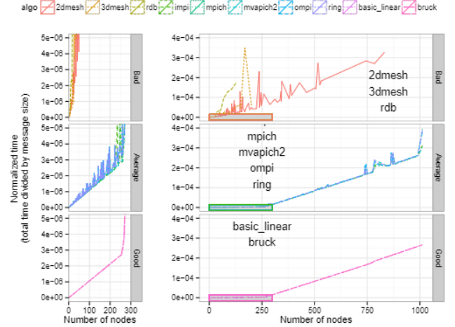
Figure 12: Evaluation of various algorithms for the MPI_Alltoall operation.
