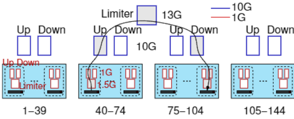
Figure 5: Modeling graphene : rectangles represent capacity constraints. Grayed rectangles show those involved in an inter-cabinet communication.
