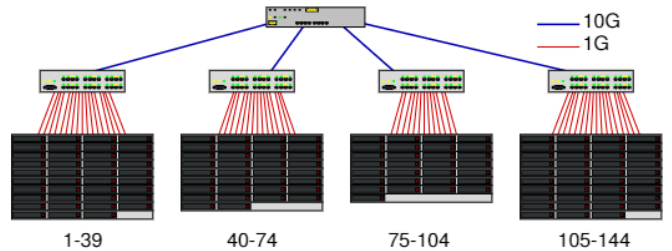
Figure 2. The graphene cluster: a hierarchical Ethernet-based cluster.
