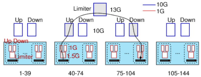
Figure 5. Modeling the graphene cluster: rectangles represent capacity constraints. Grayed rectangles represent constraints involved in a communication from node 40 to node 104.
