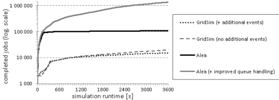
Fig. 2. Number of completed jobs during 1 hour-long simulation using different implementations of SpaceShared policy and (un)optimized queue handling.
